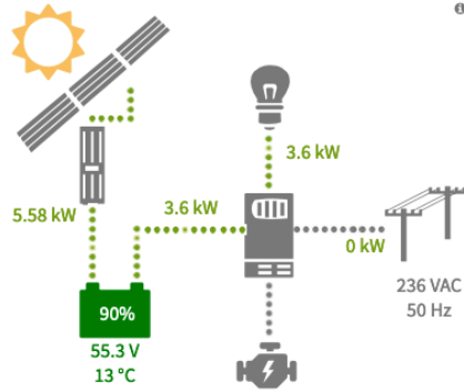
POWER FLOW
